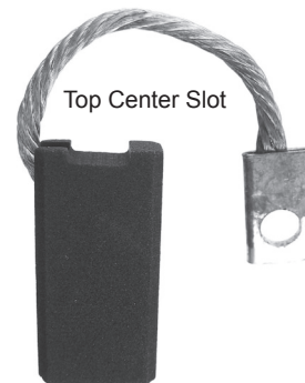
Cat. No. REP586 Size: 3/8 x 5/8 x 1 1/4 Grade Type: EG
