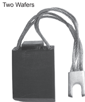
Cat. No. REP1008W Size: 1/2 x 1 5/8 x 2 1/4 Grade Type: EG
