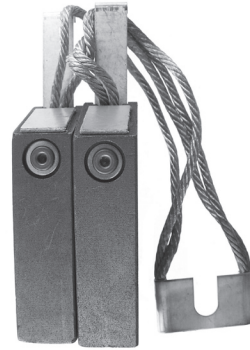
Cat. No. REP2878 Size: 1.260 x .787 x 3.125 Grade Type: G
