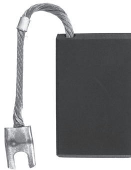
Cat. No. REP722 Size: 3/8 x 1 1/2 x 2 1/2 Grade Type: EG
