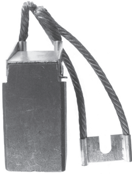
Cat. No. REP1020 Size: 1 1/2 x 1 1/2 x 3 Grade Type: G
