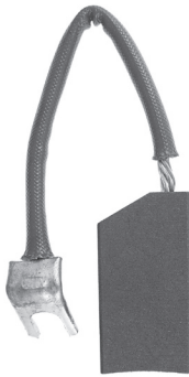
Cat. No. REP1444 Size: 5/8 x 5/16 x 1 1/4 Grade Type: EG
