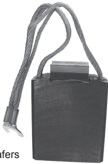
Cat. No. REP599W Size: 1/2 x 1 1/2 x 1 3/4 Grade Type: EG
