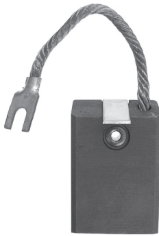
Cat. No. REP415 Size: 1/2 x 1 1/4 x 2 Grade Type: EG
