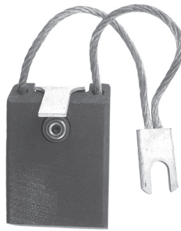
Cat. No. REP642 Size: 1/2 x 1 1/2 x 2 1/4 Grade Type: EG
