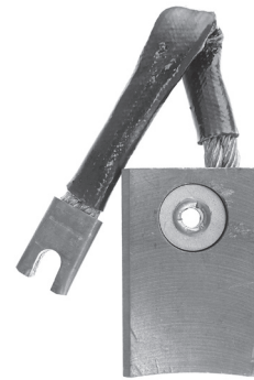
Cat. No. REP458W Size: 1 1/2 x 5/8 x 2 1/4 Grade Type: MG
