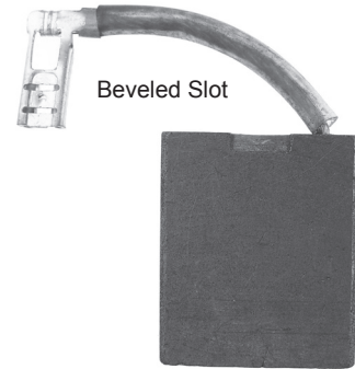
Cat. No. REP623W Size: 19/64 x 7/8 x 1 1/32 Grade Type: G
