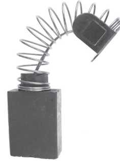
Cat. No. REP1267 Size: 3/8 x 3/4 x 1 1/8 Grade Type: G
