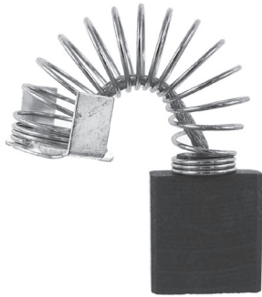
Cat. No. REP676W Size: 1/4 x 5/8 x 13/16 Grade Type: EG
