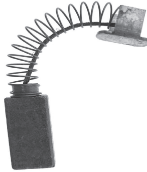
Cat. No. REP2802 Size: 3/16 x 5/16 x 3/4 Grade Type: EG
