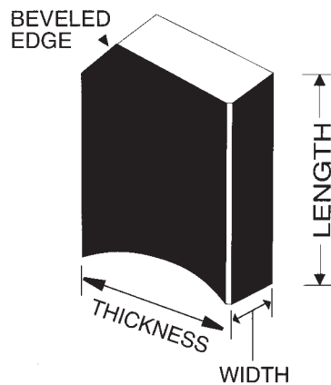
Slip Ring Brush
