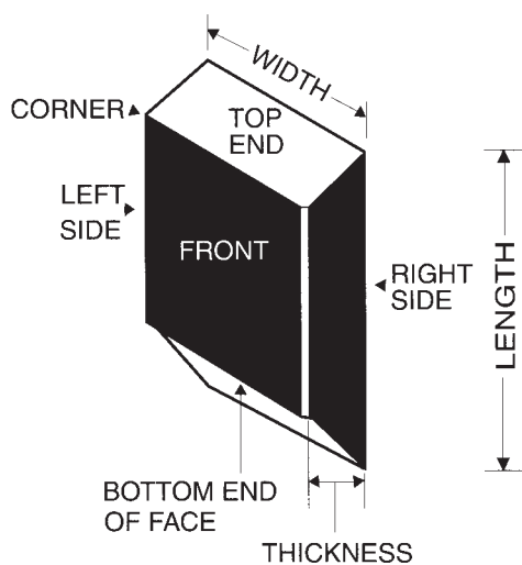
Commutator Brush (With Bevels)
