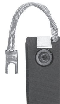
Cat. No. REP419 Size: 1/2 x 1 x 2 Grade Type: G
