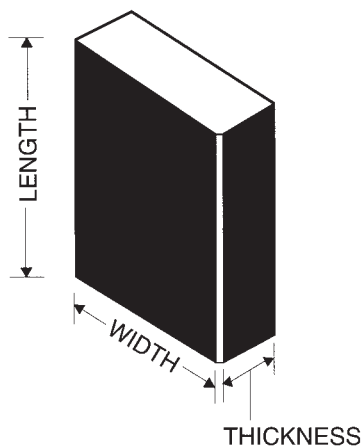
Commutator Brush (No Bevels)
