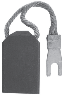
Cat. No. REP767 Size: 3/8 x 1 x 1 25/32 Grade Type: EG
