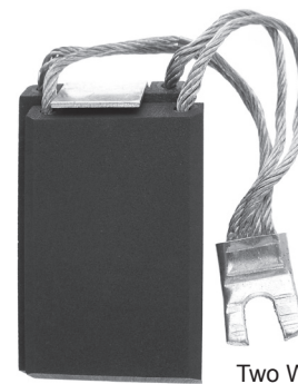
Cat. No. REP521W Size: 3/4 x 1 1/2 x 2 3/4 Grade Type: EG
