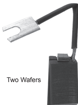
Cat. No. REP311W Size: 3/8 x 3/4 x 1 1/2 Grade Type: EG
