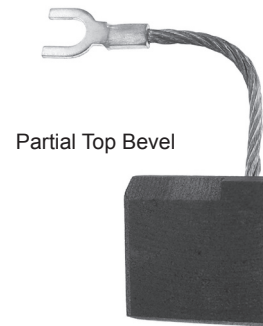
Cat. No. REP551W Size: 3/8 x 1 x 1 1/16 Grade Type: EG
