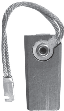
Cat. No. REP353 Size: 1 1/4 x 3/4 x 2 3/4 Grade Type: G
