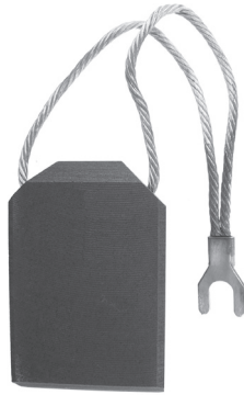
Cat. No. REP992A Size: 1/2 x 1 3/4 x 2 3/4 Grade Type: EG
