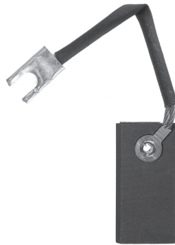
Cat. No. REP426W Size: 1 x 1/2 x 1 7/8 Grade Type: EG
