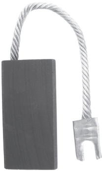
Cat. No. REP482 Size: 5/8 x 1 1/4 x 2 1/2 Grade Type: EG
