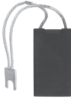
Cat. No. REP686 Size: 1/2 x 1 1/2 x 2 3/4 Grade Type: EG
