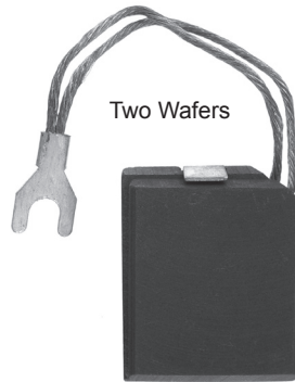
Cat. No. REP402W Size: 1/2 x 1 1/2 x 2 Grade Type: EG
