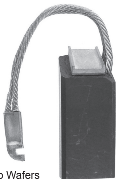
Cat. No. REP1092 Size: 1 x 1 1/4 x 3 1/4 Grade Type: EG
