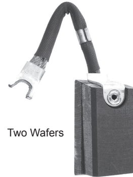
Cat. No. REP465W Size: 7/8 x 3/4 x 1 5/8 Grade Type: EG
